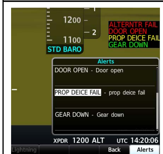
PROP DE-ICE FAIL ALERT & ANNUNCIATION
