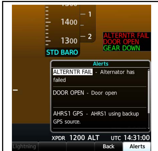
ALTERNATOR FAIL ALERT & ANNUNCIATION
