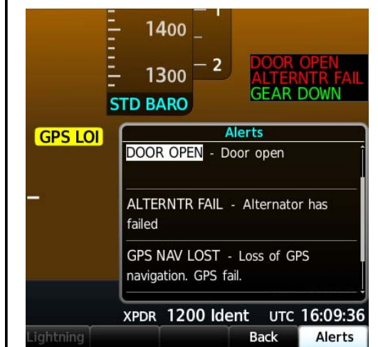
DOOR OPEN ALERT & ANNUNCIATION
