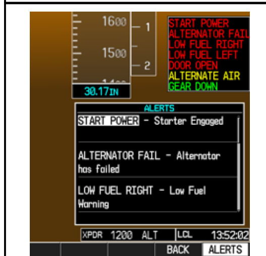
START POWER - ALERT & ANNUNCIATION
