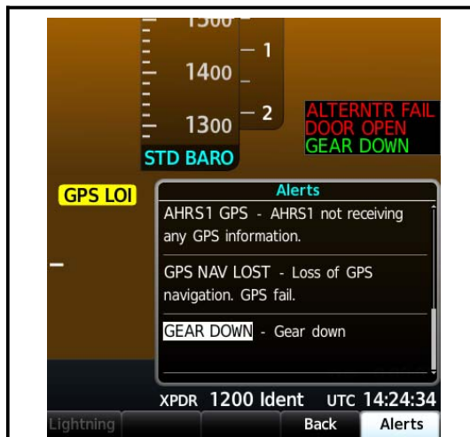
GEAR DOWN - ALERT & ANNUNCIATION
