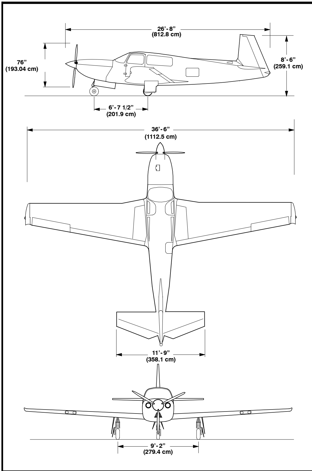
FIGURE 1-1 THREE VIEW
