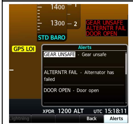
GEAR UNSAFE - ALERT & ANNUNCIATION
