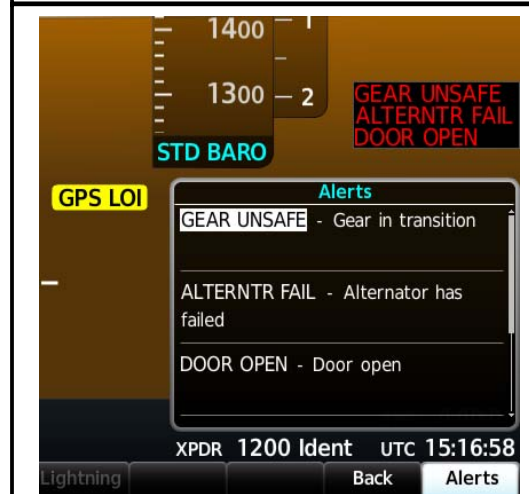
GEAR UNSAFE - ALERT & ANNUNCIATION "IN TRANSITION"
