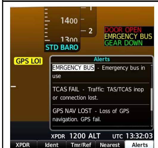
EMERGENCY BUS ALERT & ANNUNCIATION
