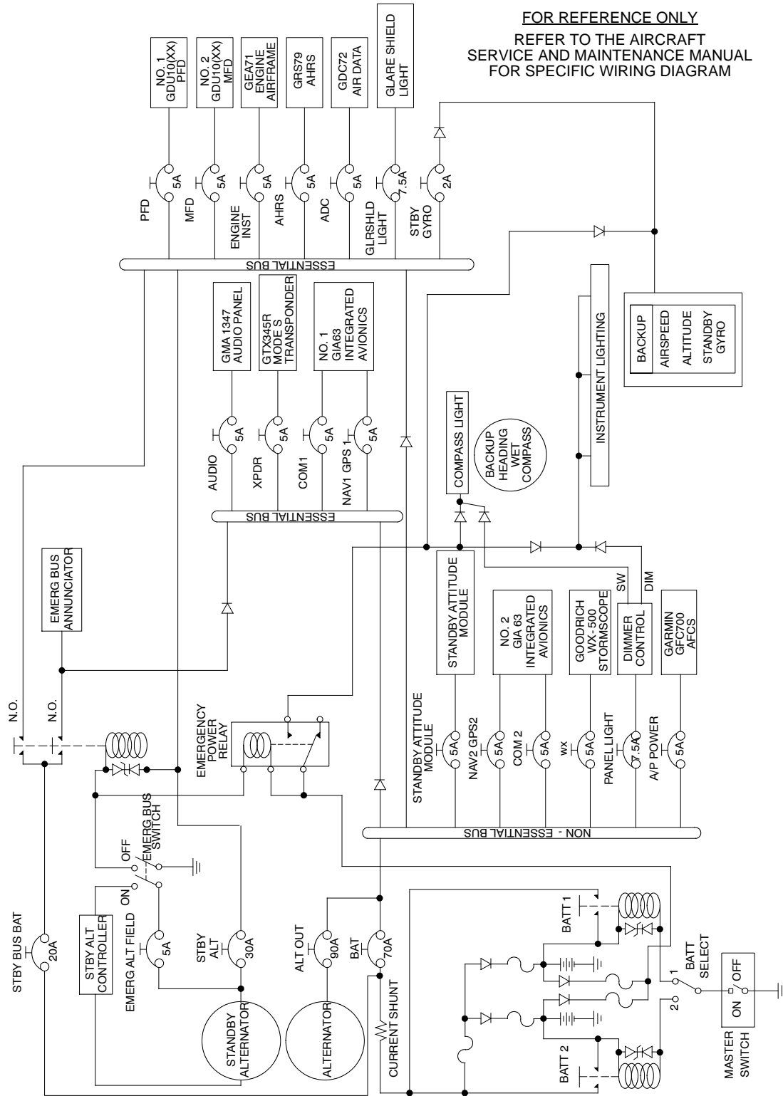
Figure 7-8 M20V POWER SUMMARY - GENERIC SYSTEM SHOWN
