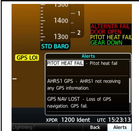
PITOT HEAT FAIL ALERT & ANNUNCIATION
